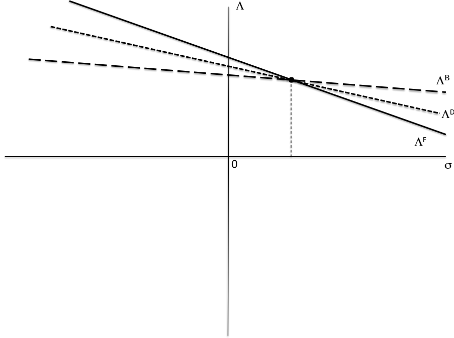
Figure 8: Single crossing between \Lambda^F , \Lambda^B and \Lambda^D
