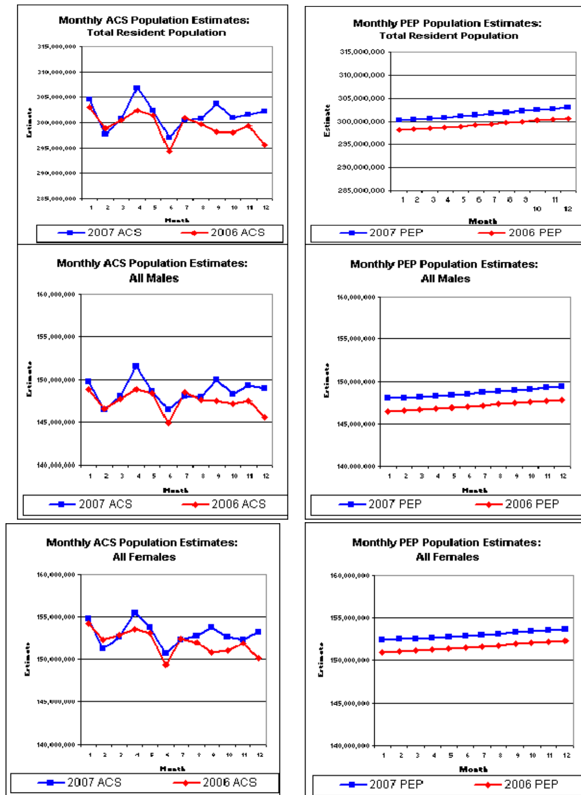
Figure 1--Comparison of Monthly Resident Population Estimates from the American Community Survey (ACS) and Population Estimates Program (PEP), 2006 and 2007: Total Population and by Sex
